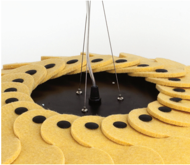
Top of lighting panel with suspension wires. Three adjustable length wires join into a central wire for easy hanging.
